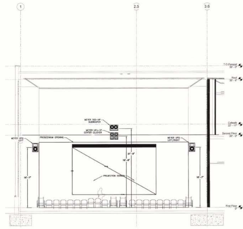
1 LEFT/CENTER/RIGHT/SUBWOOFER NORTH ELEVATION SCALE: 1/4" = 1'-0"
